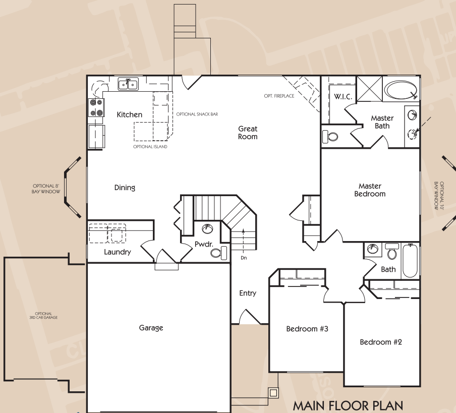
(Elevation B)
